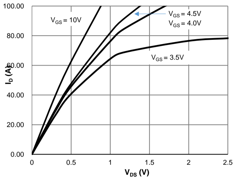
Figure 1: Saturation Characteristics
